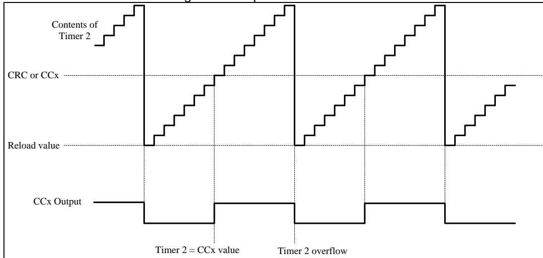
Fig. 7-1: Compare mode 0 function
