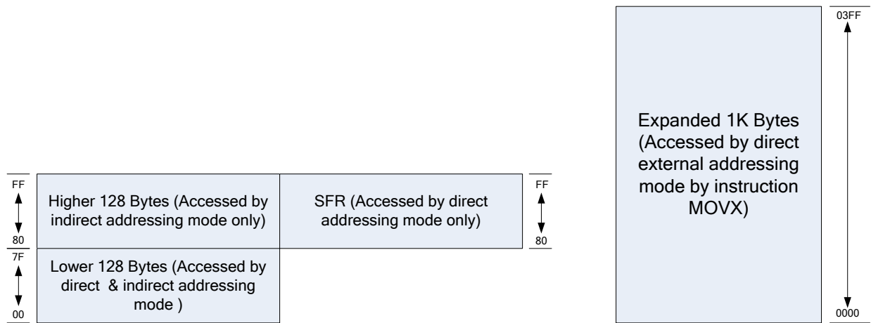
Fig. 3-3: RAM architecture
