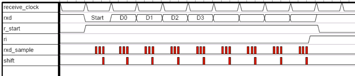
Fig. 8-4: Receive mode 1 for Serial 0
